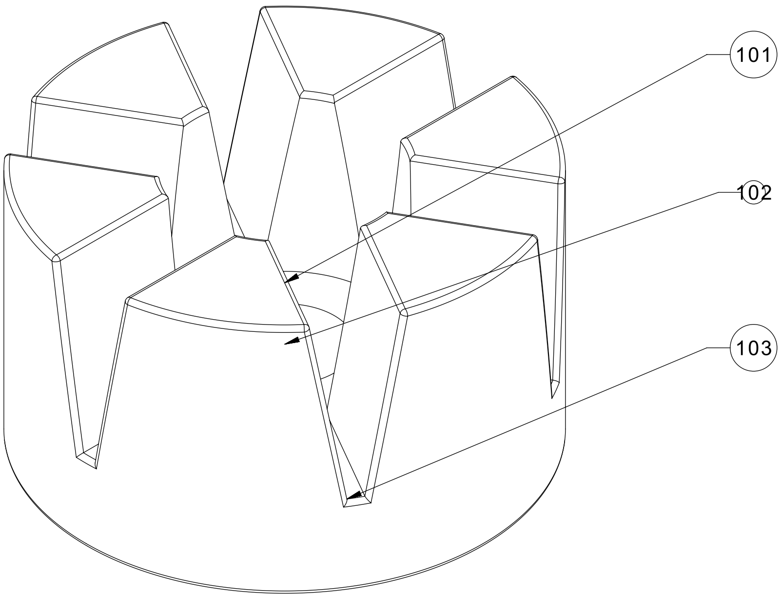
ISOMETRIC VIEW
