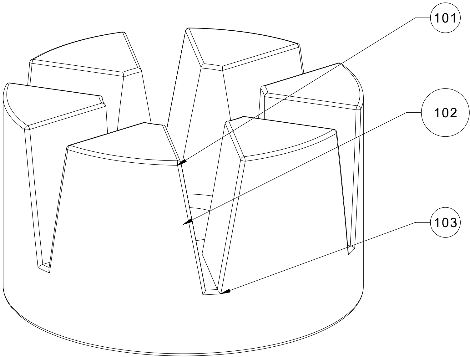
ISOMETRIC VIEW
